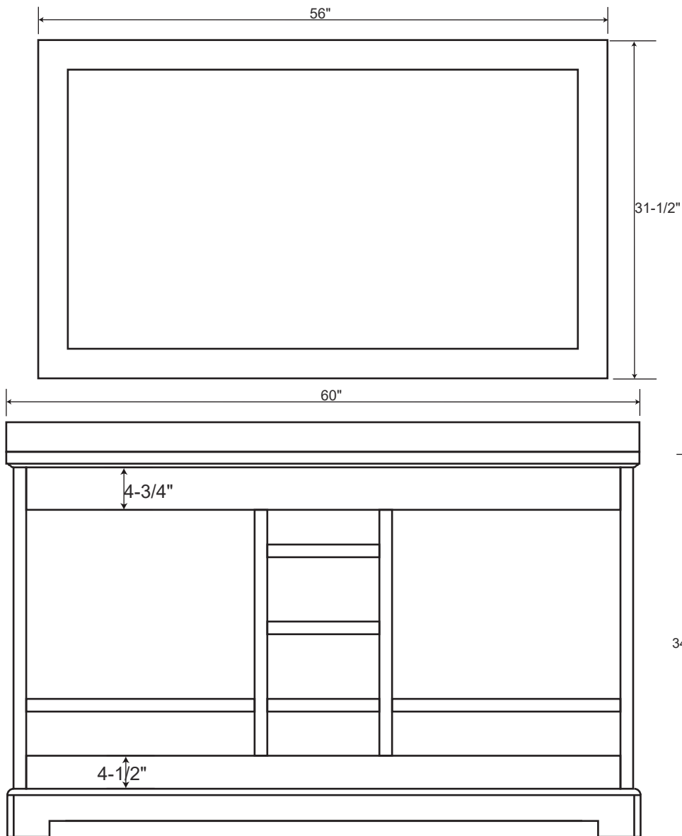
60" Back View
