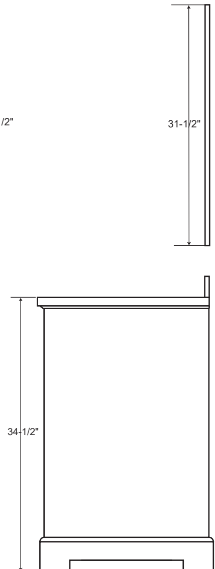
60" Side View
