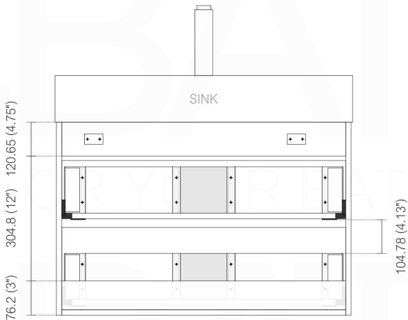
. BACK ELEVATION
