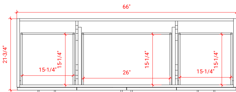
PLAN VIEW
