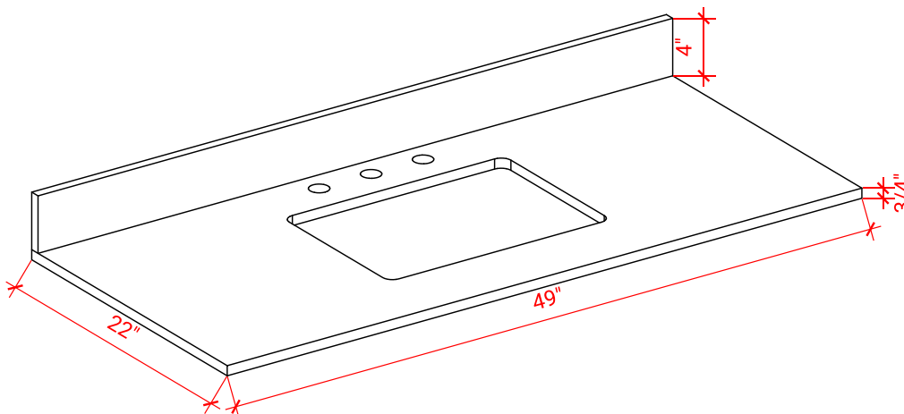
THREE DIMENSIONAL COUNTERTOP VIEW
