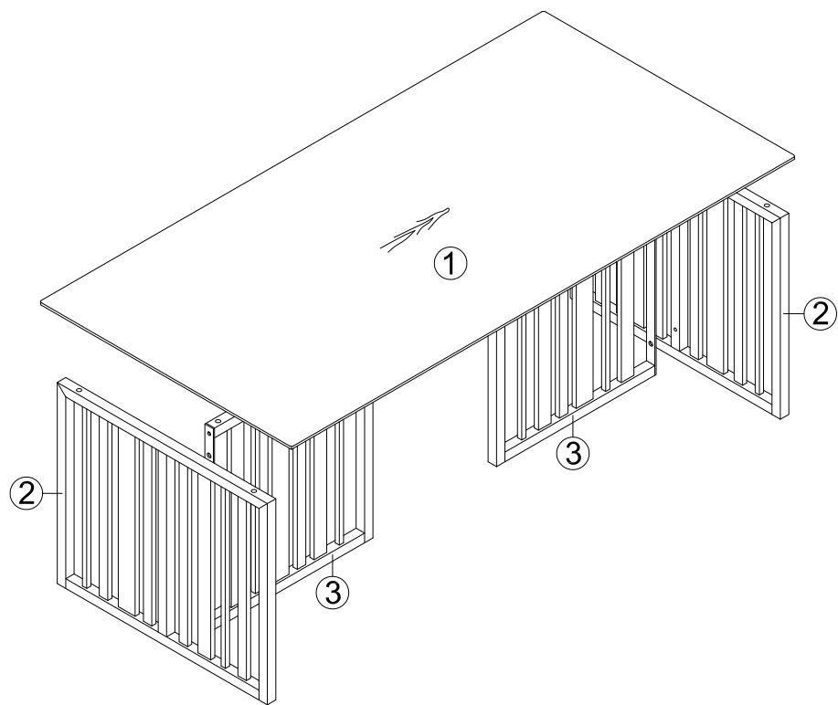
Exploded View
