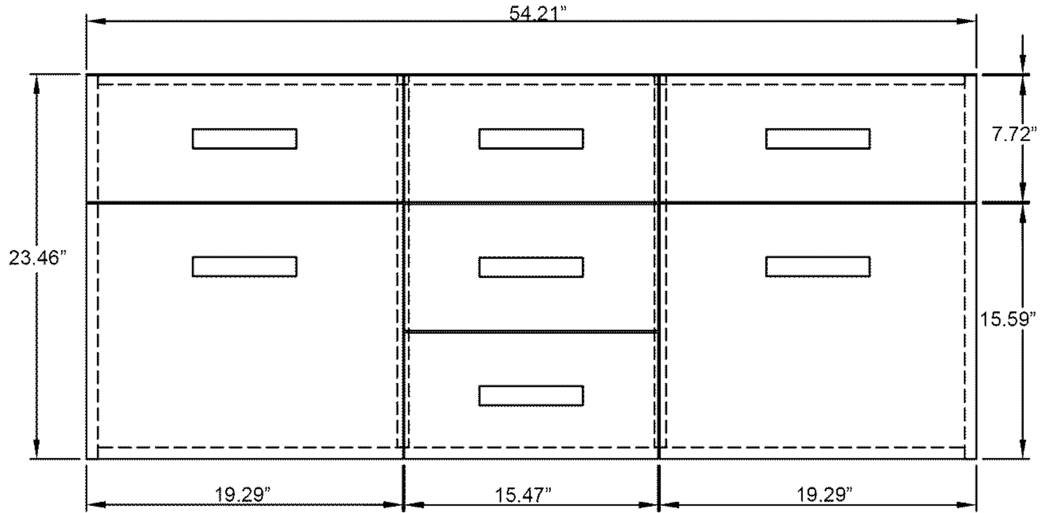
Front View
