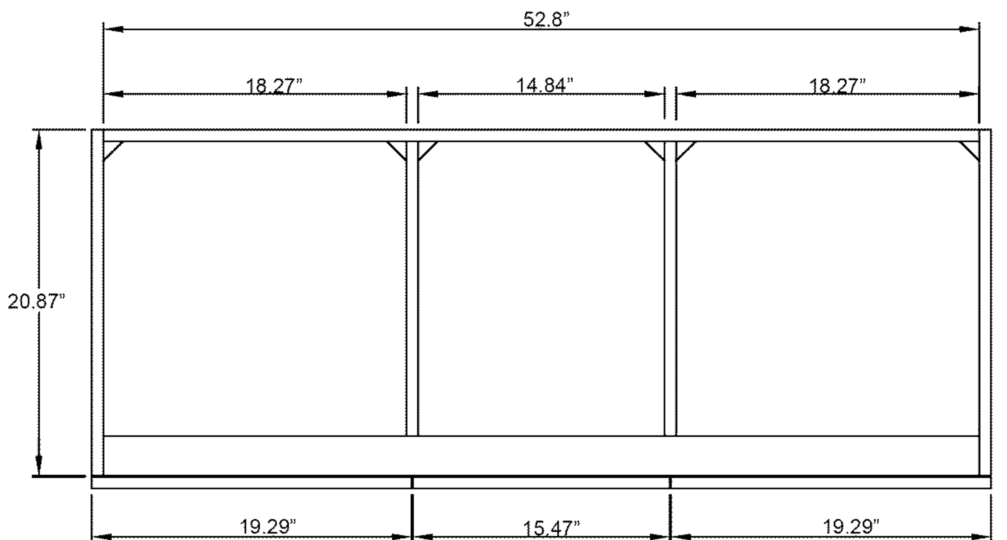
Top View
