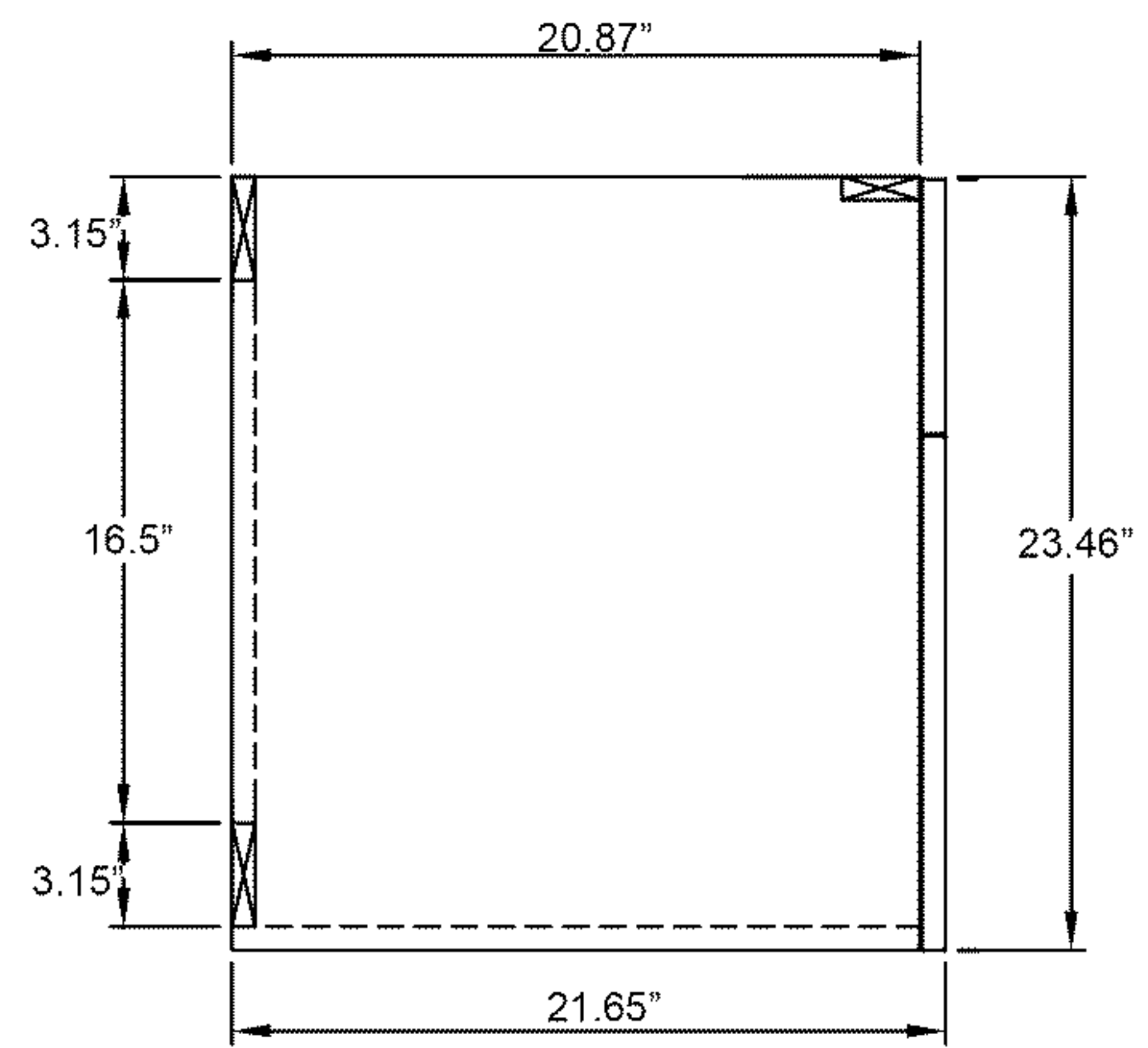
Side View
