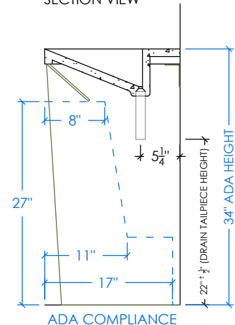
SECTION VIEW
