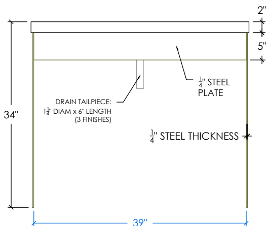
FRONT ELEVATION
