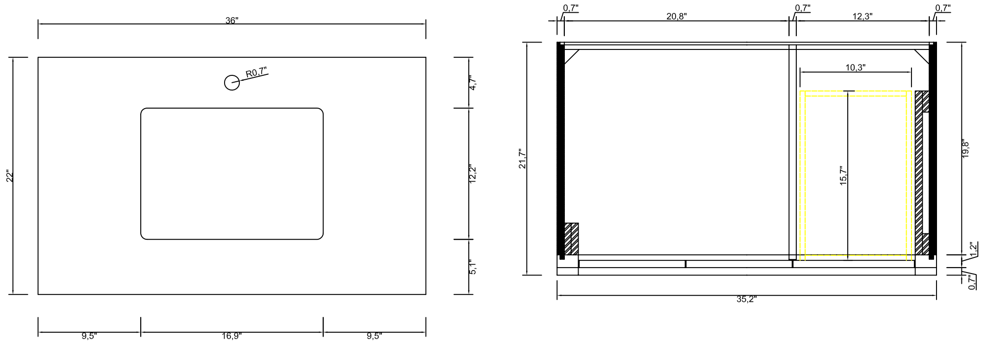
TOP VIEW
