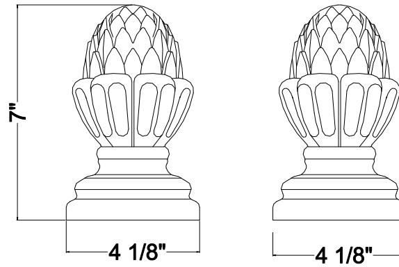
ITEM NUMBER:FIN04X07BL 4 1/8"OD x 7"H Blackthorne Finial
