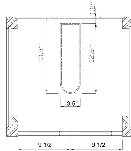
B - B SECTION
