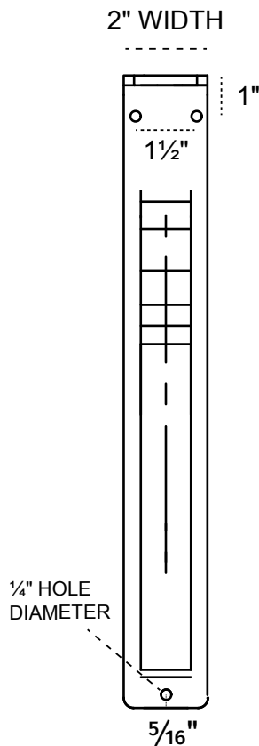
FRONT PROFILE
