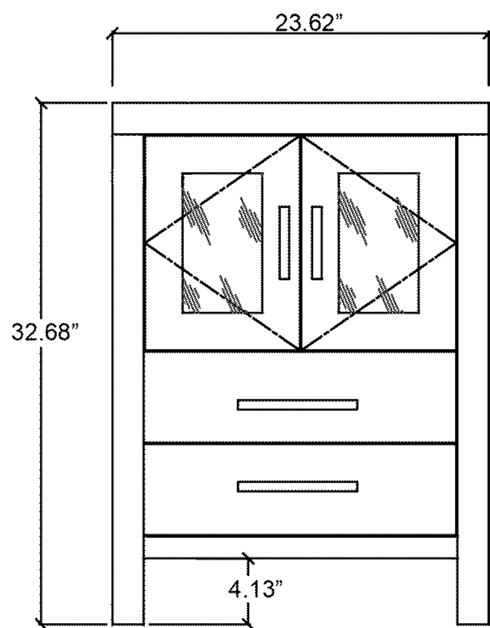
Front View
