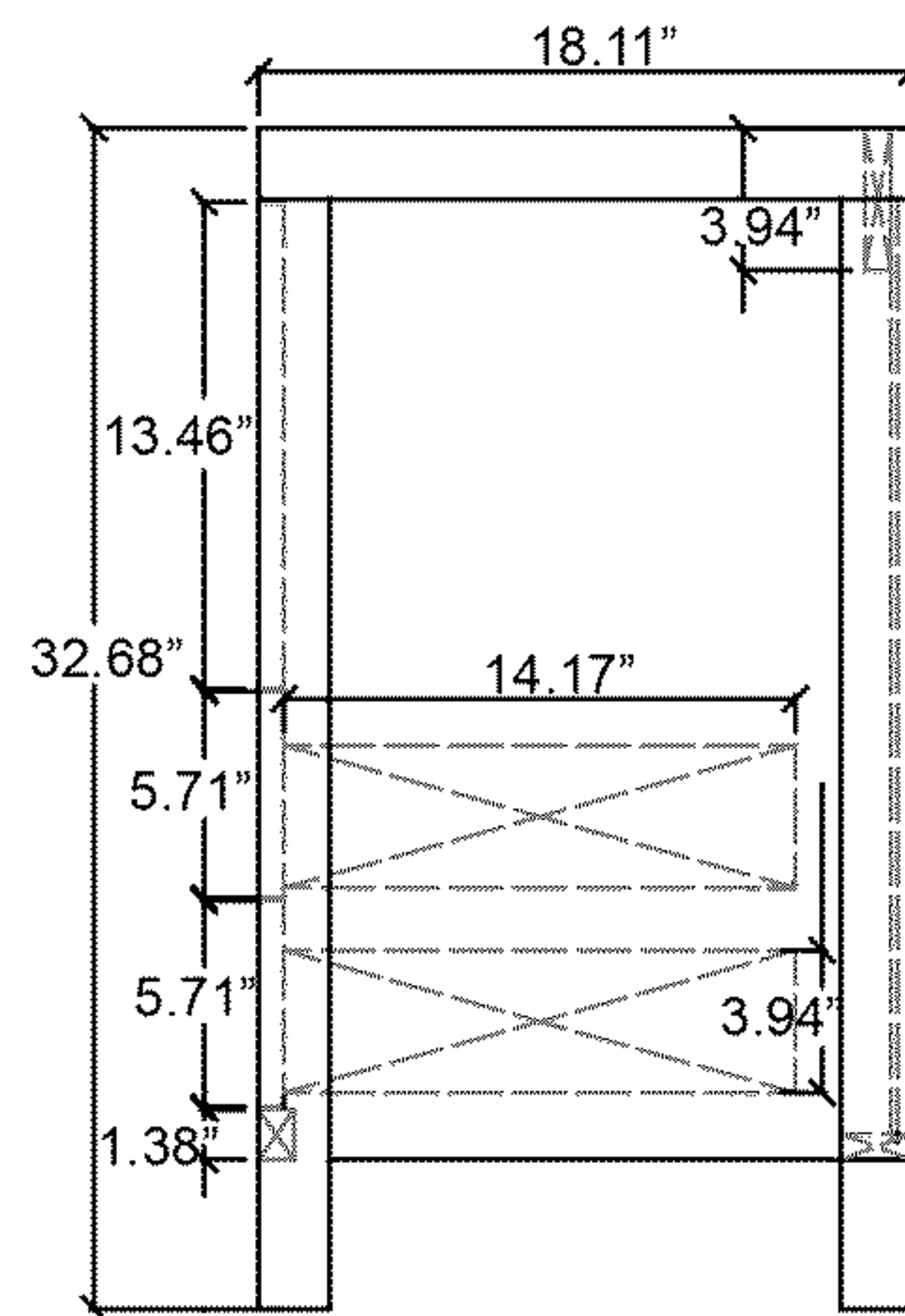
Side View
