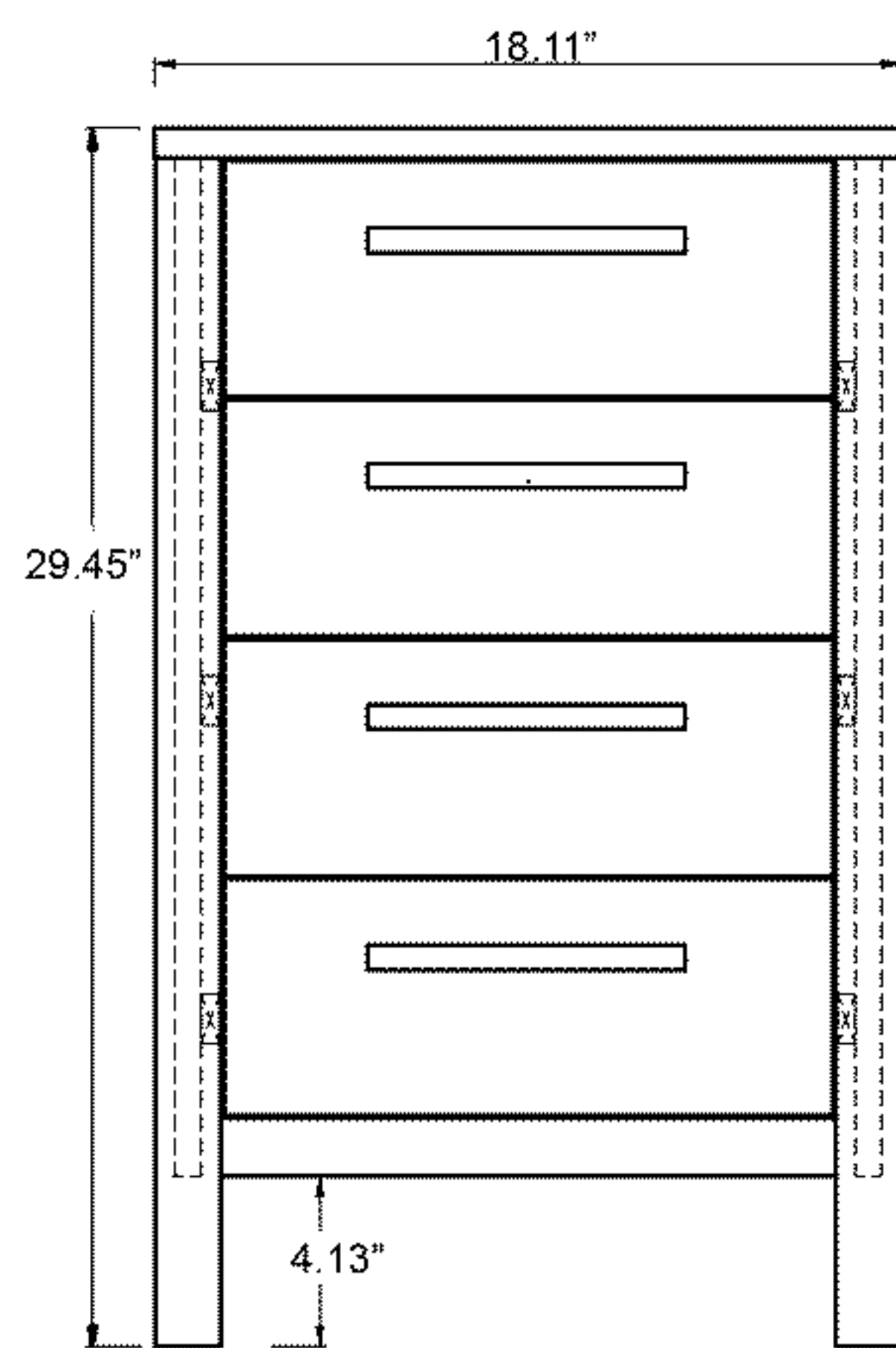
Front View
