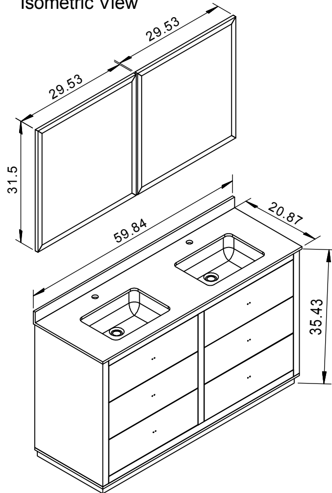
Isometric View
