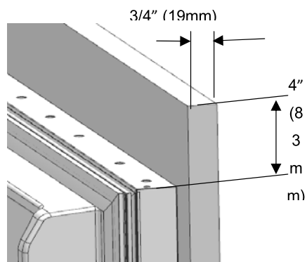
Assembly dimension between Wood panel and freezer door
