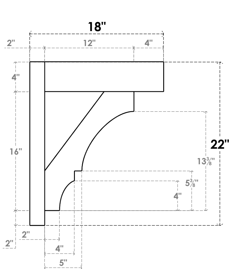
SIDE PROFILE
