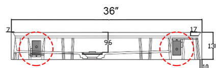
Metal Support Front View
