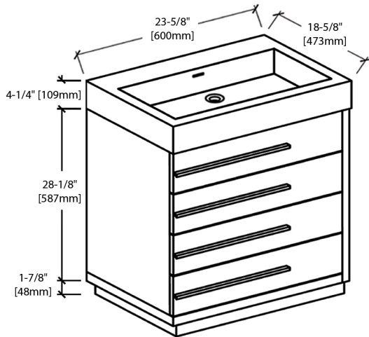
VANITY FRONT VIEW (V8005 24)
