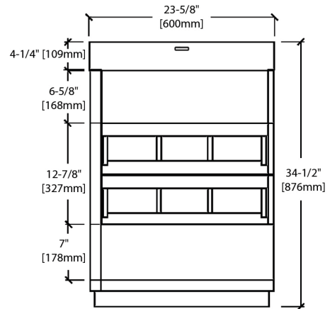
VANITY BACK VIEW (V8005 24)
