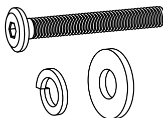
ALLEN KEY BOLT: M8 X 50mm - QTY 8 LOCK WASHER: Ø12 / Ø8 X 1.5mm - QTY 8 WASHER: Ø19 / Ø8 X 1mm - QTY 8 QTY 8 SETS
