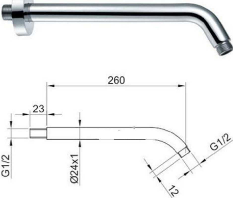
Φ24×1.0×260(mm) Brass shower arm
