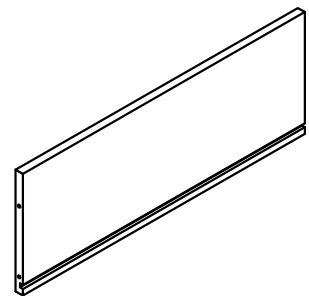
LARGE DRAWER BACK QTY 4
