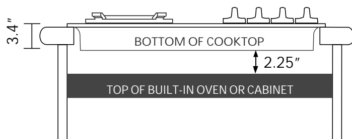
FRONT VIEW (INSTALLED)
