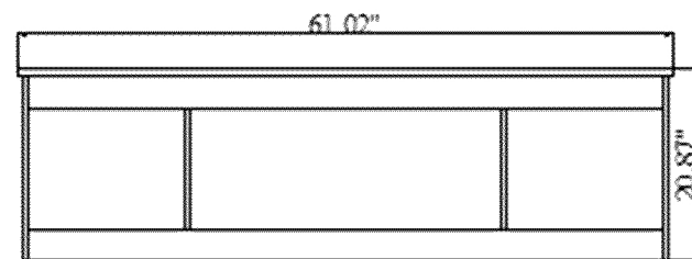
BACK VIEW
