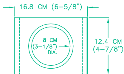
TOP VIEW OF STAND
