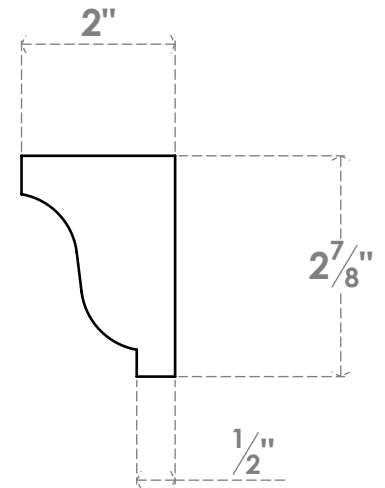
SIDE PROFILE
