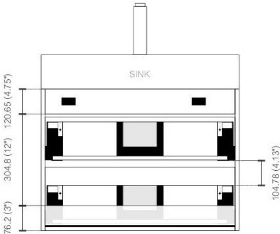
. BACK ELEVATION
