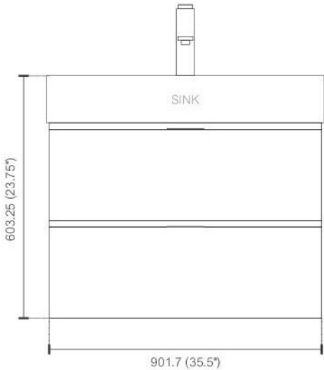
. FRONT ELEVATION
