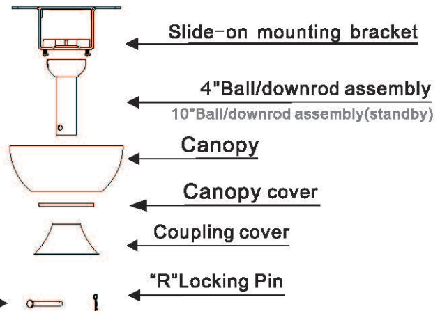
Fan-motor assembly
