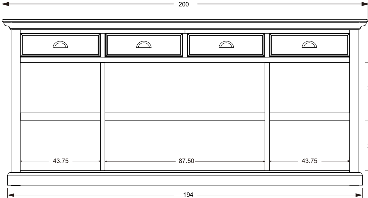
OPEN FRONT VIEW
