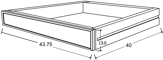
LARGE DRAWER DETAIL
