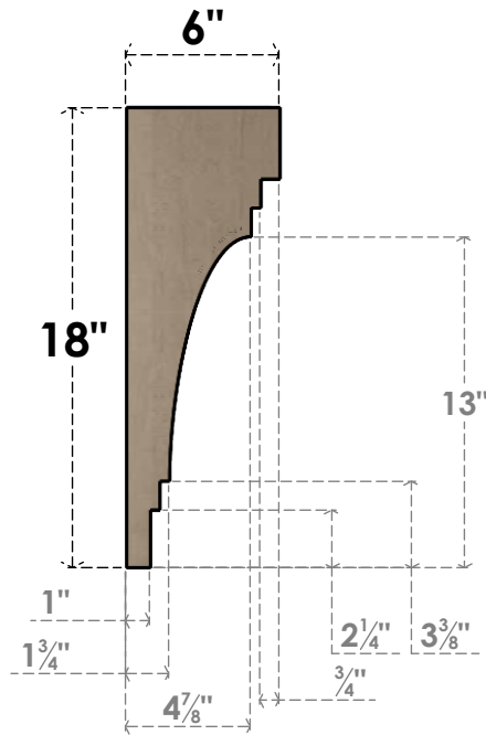
SIDE PROFILE
