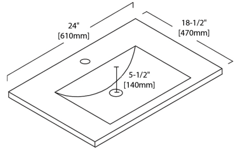
TOPMOUNT SIDE VIEW (C04 2418)
