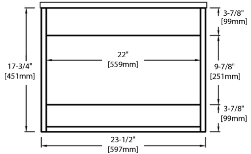
24" VANITY BACK VIEW (V8008 24 01)
