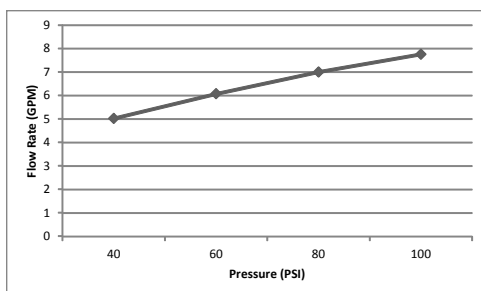
4024B Flow Rate (GPM) Vs Pressure (PSI)*
