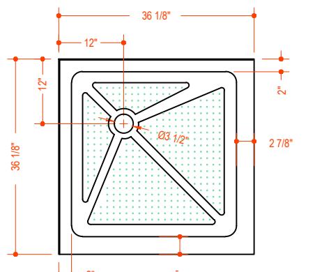
MODEL VG06019XXX3240*
