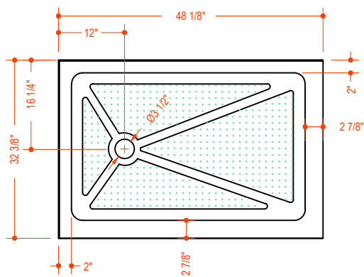
MODEL VG06019XXX3232
