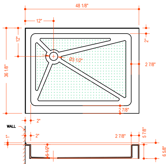
MODEL VG06019XXX3648
