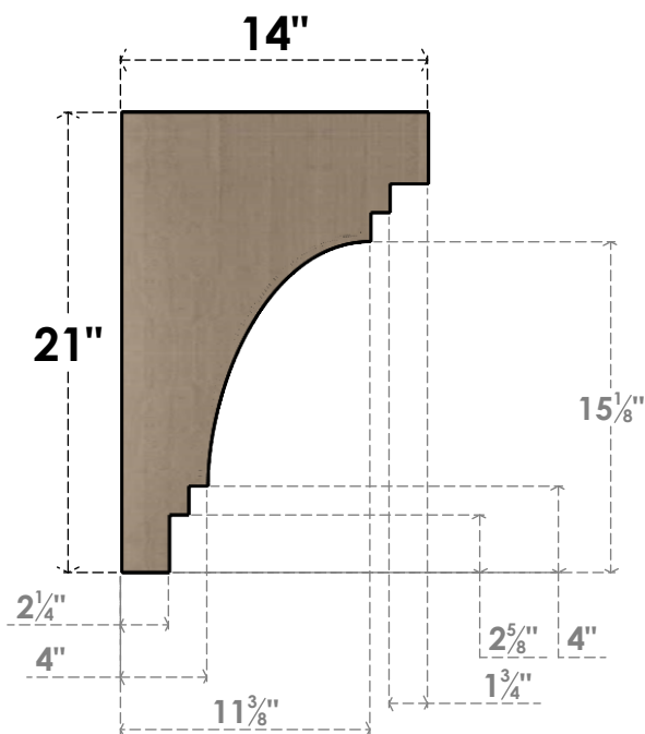
SIDE PROFILE
