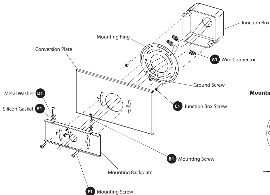
FIG. 2 MOUNT ON JUNCTION BOX
