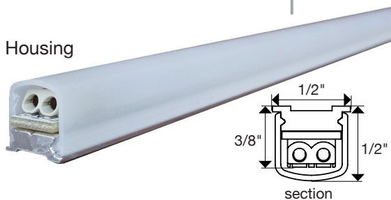
Angled Housing
