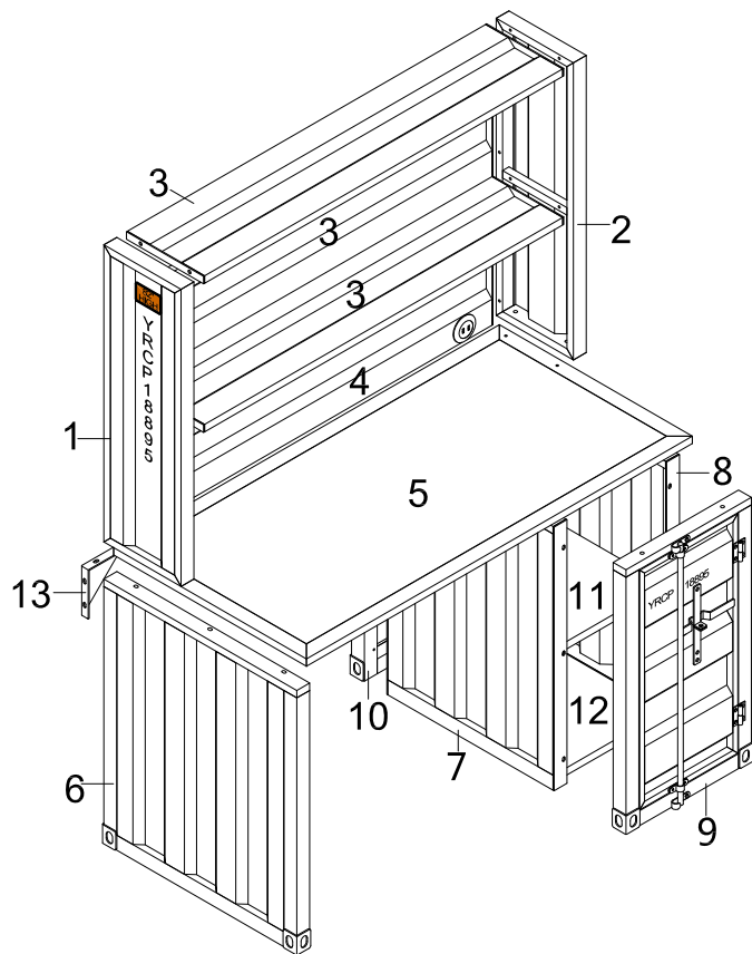
Exploded View
