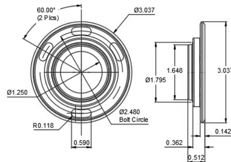
IFSS-CER-FLANGE Detail
