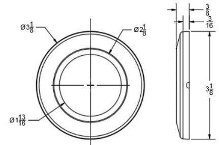
ICSS-CCR-COVER Detail
