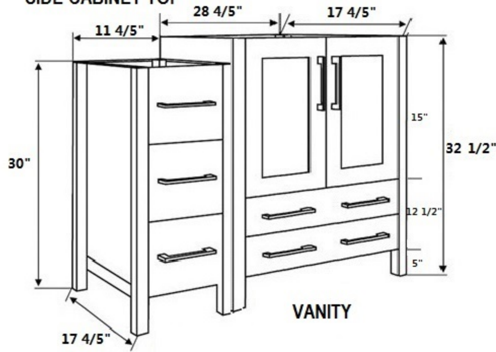
SIDE CABINET
