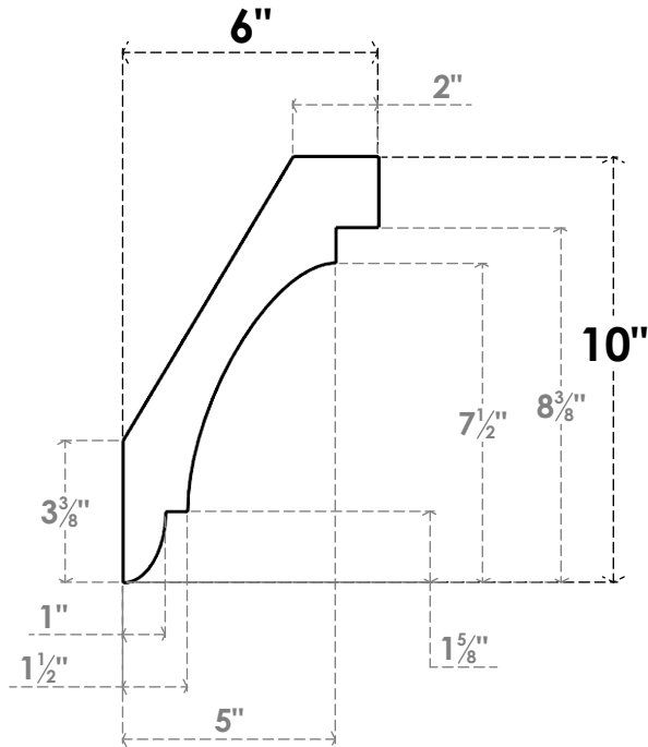
SIDE PROFILE
