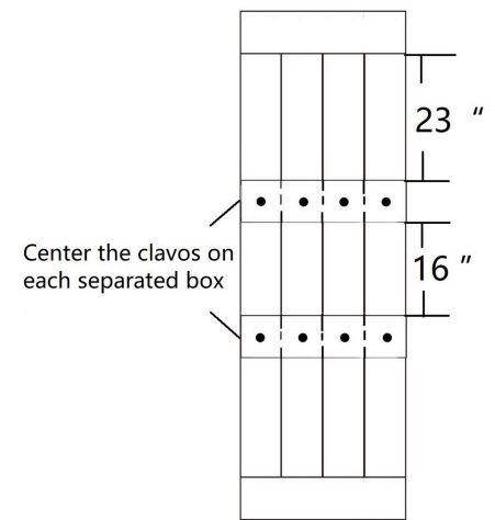
Assembled Door
