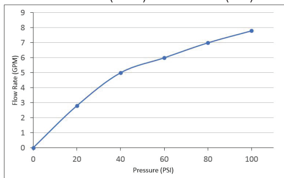
V-2300B Flow Rate (GPM) Vs Pressure (PSI) For Tub Port*
