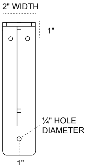
FRONT PROFILE
