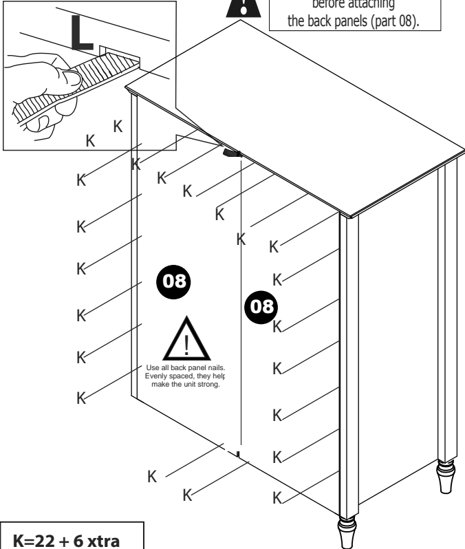
Back Panel Nail
