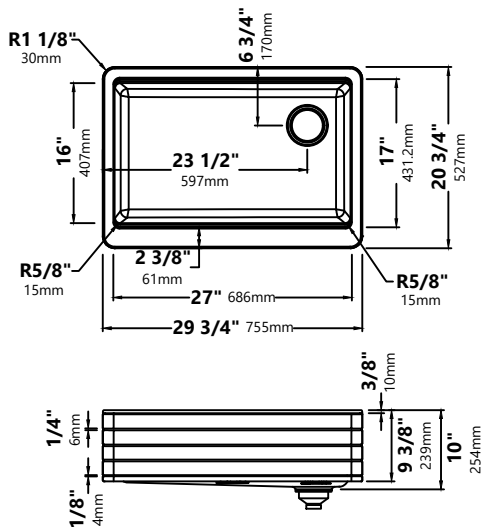
KGF12-30 29\ 3/4" \times 20\ 3/4" \times 9\ 3/8" Min Cabinet Size: 33"
