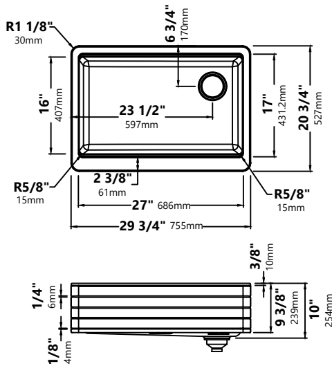
KGF11-30 29\ 3/4" \times 20\ 3/4" \times 9\ 3/8" Min Cabinet Size: 33"
