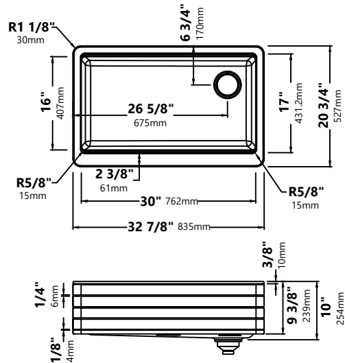
KGF12-33 32\ 7/8" \times 20\ 3/4" \times 9\ 3/8" Min Cabinet Size: 36"
