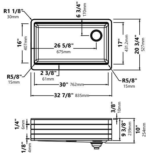
KGF11-33 32\ 7/8" \times 20\ 3/4" \times 9\ 3/8" Min Cabinet Size: 36"
