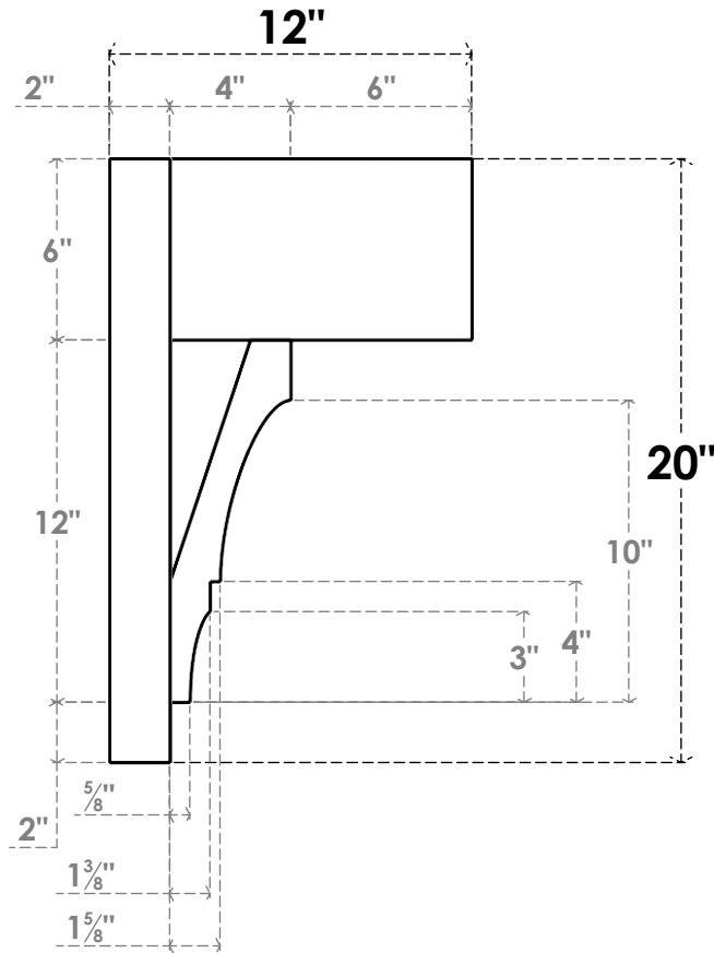
SIDE PROFILE
