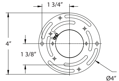
Back Plate Dimensions
