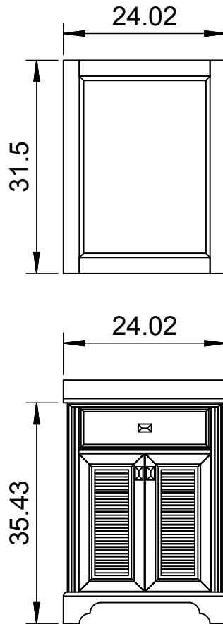
Front View
