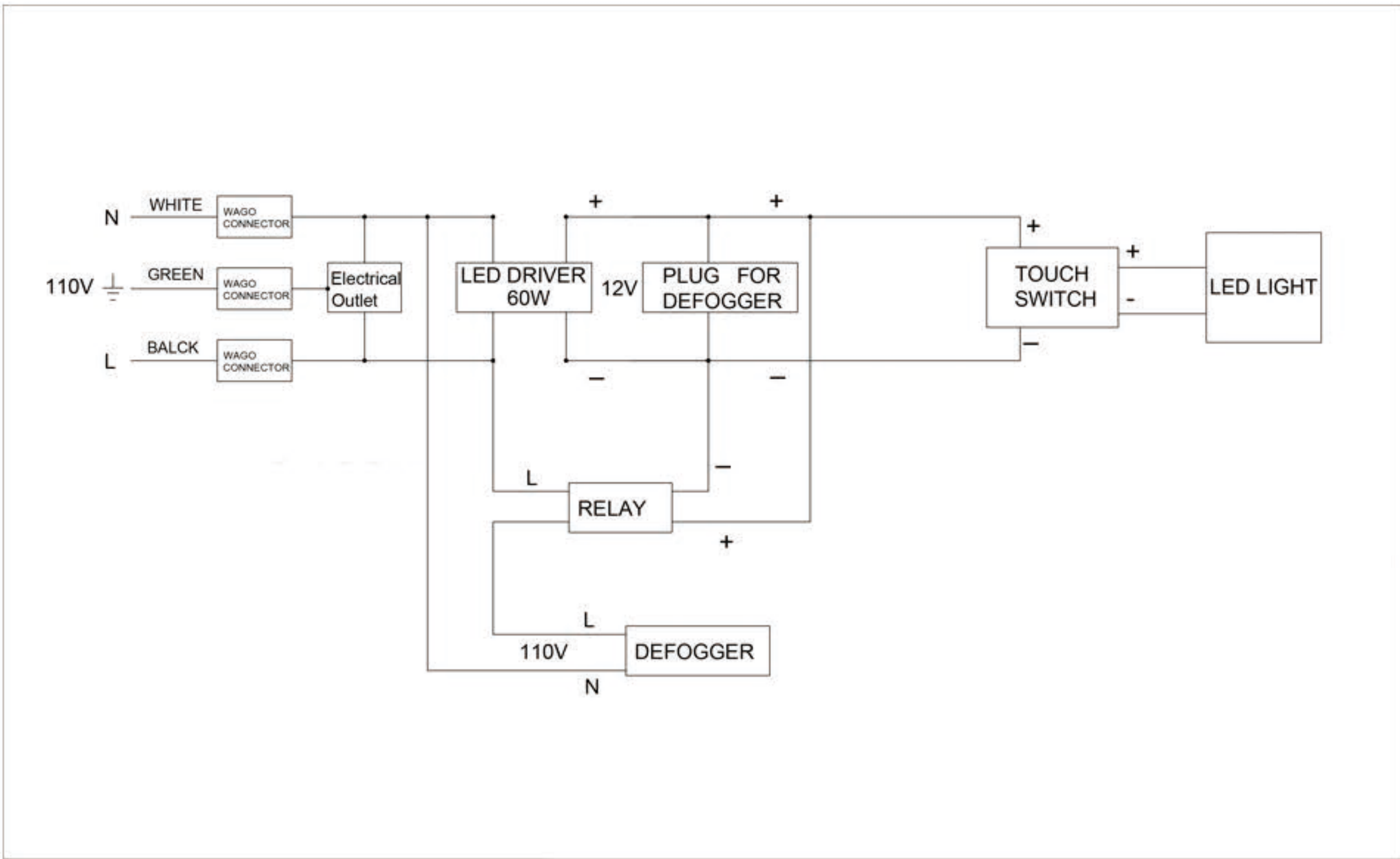
Circuit Diagram
