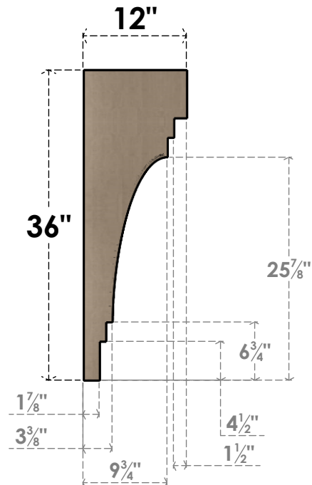
SIDE PROFILE
