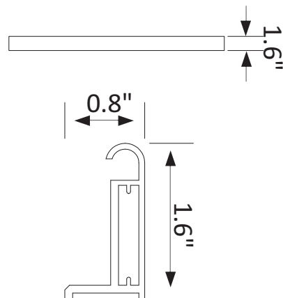
Aluminum section
