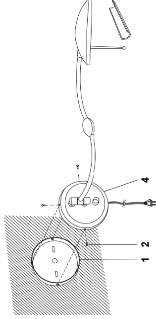
BULB / AMPOULE MAX 100WATT-T3 (DL100Q3) (included)
